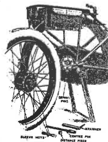
Back Detachable Wheel Removed.
