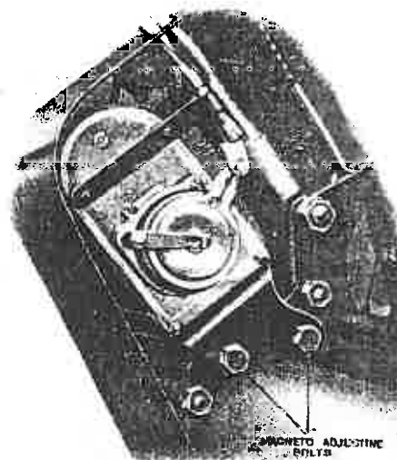
A.J.S. Magneto Adjustment.
