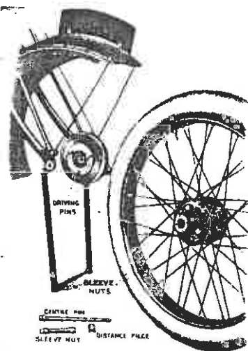
Showing Front Wheel detached and its interchangeability with Rear Wheel.
