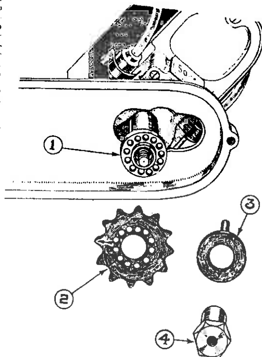
Magneto Timing—Vernier Adjustment.
