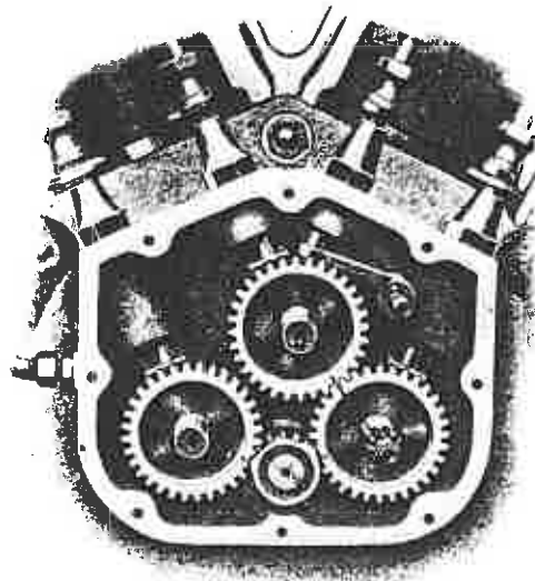
Arrangement of Timing Gear 7 h.p. A.J.S.
